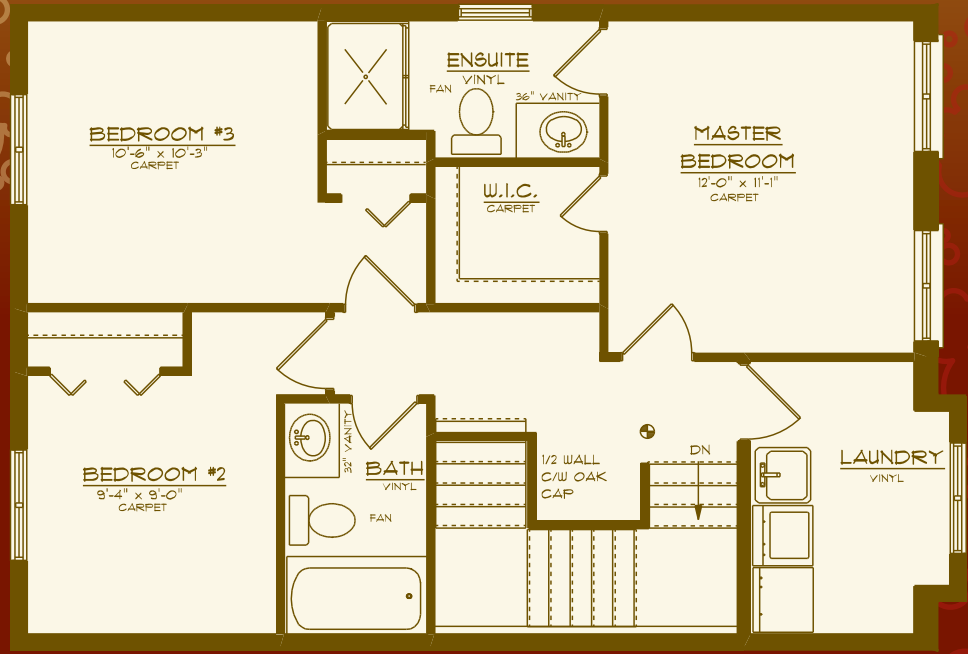
Upper Floor 789 Sq. Ft.
